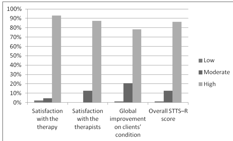
Figure 5: Bar Chart Showing Participants' Satisfaction with Therapy
